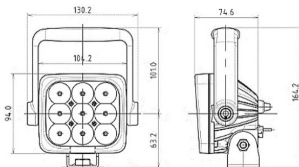
Pictured above is the Handle and Switch measurements
